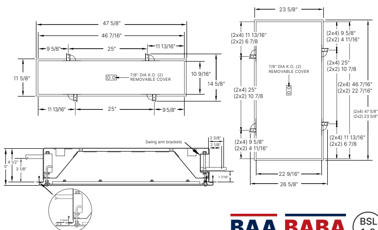
Ceiling Grid / Flange Design
