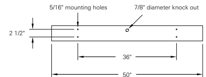
4' Fixture
