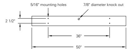
4' Fixture
