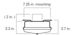
M16377/11C-77.4SSL Standard mount fixture with white diffusing lens and two LED arrays
