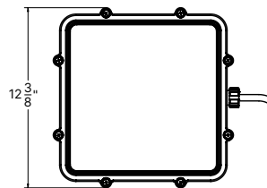
5/16" dia. mounting holes
